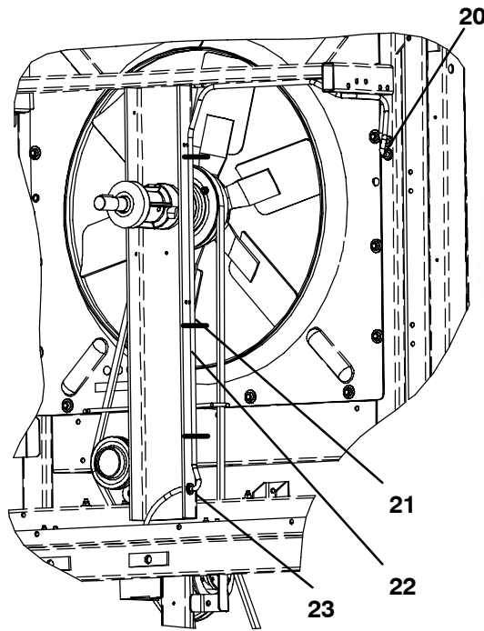
CURBSIDE VIEW
